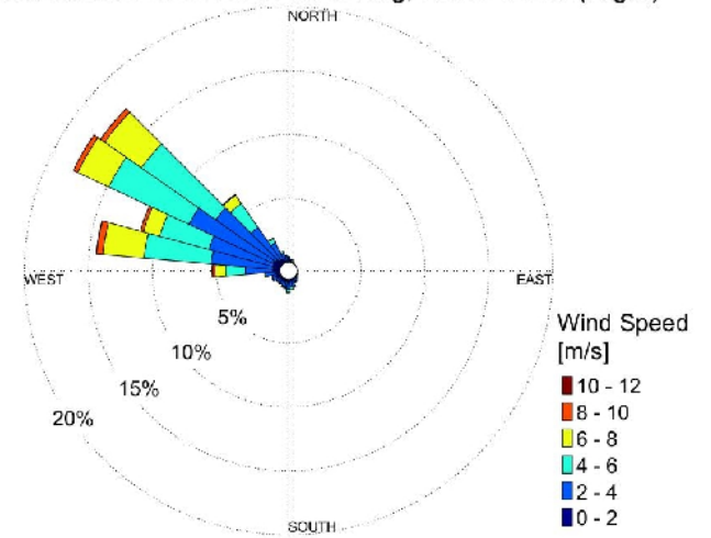
Wind Record 2002-2012 June-Aug, 20:00-04:00 (Night)
