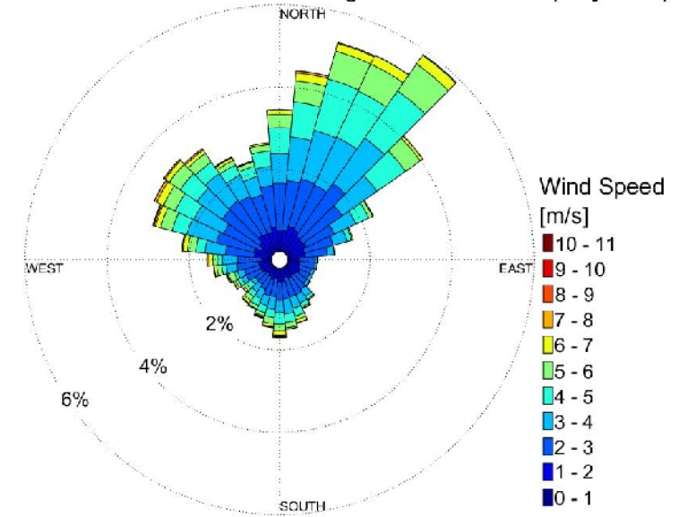
Wind Record 2002-2012 June-August 08:00-14:00 (Day time)
