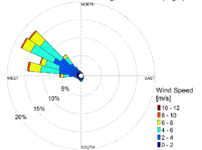
Wind Record 2002-2012 June-Aug, 20:00-04:00 (Night)
