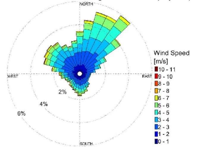
Wind Record 2002-2012 June-August 08:00-14:00 (Day time)
